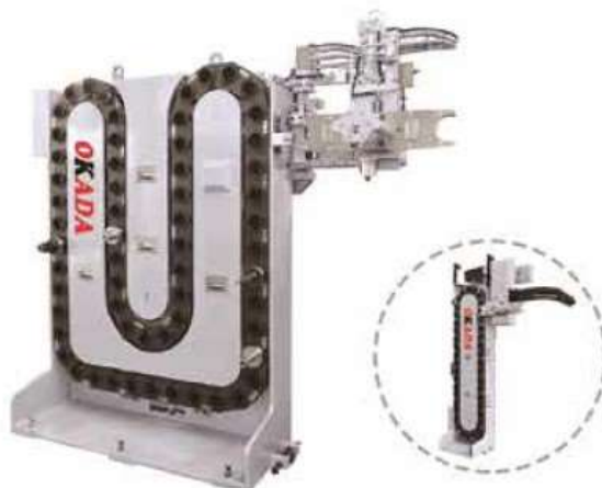
Hydraulic Swing Type Tool Magazine (32T,40T,60T,80T,120T,180T)
